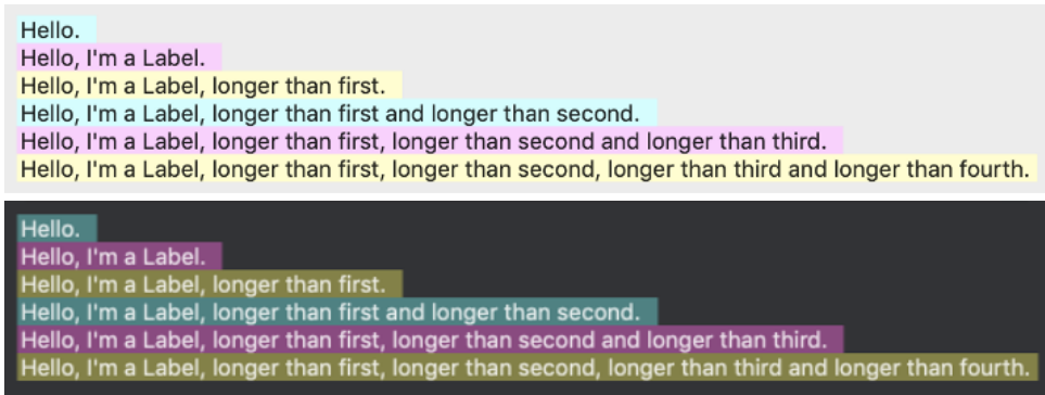
Figura 26.1: Controles Label .
